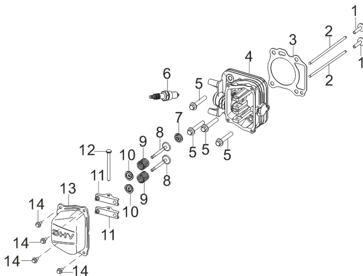
FIG.3 HEAD SUBASSEMBLY, CYLINDER / PLUG,SPARK (E03)
