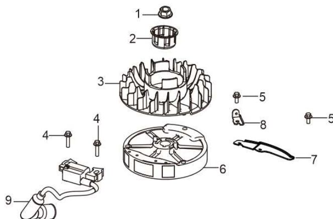
FIG.7 FLYWHEEL / IMPELLER / STARTER PULLEY / IGNITION COIL (E07)
