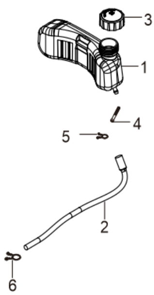
FIG.14 TANK ASSY, FUEL F03)
