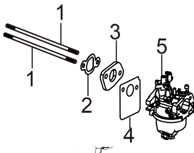
FIG.6 CARBURETOR ASSY. (E06)
