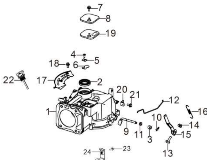
FIG.1 CRANKCASE. / GEAR ASSY, GOVERNOR. (E01)
