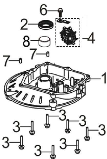
FIG.2 COVER SUBASSEMBLY, CRANKCASE (E02)
